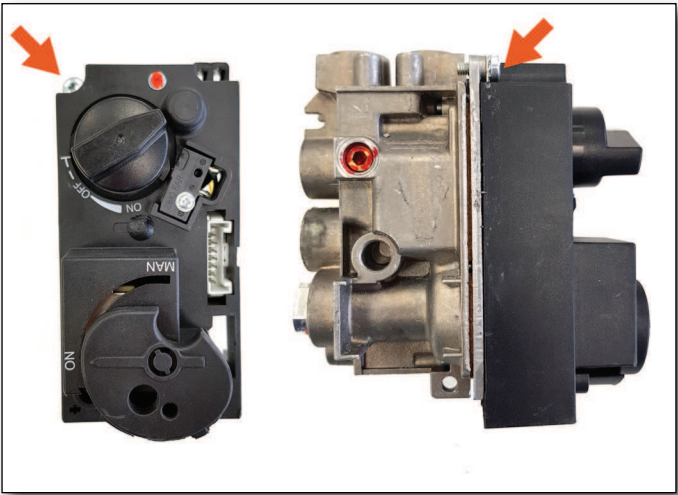
Figure A-3: Torx screw
