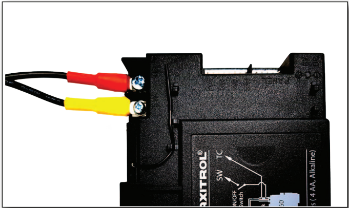
Figure A-6: Wiring receiver
