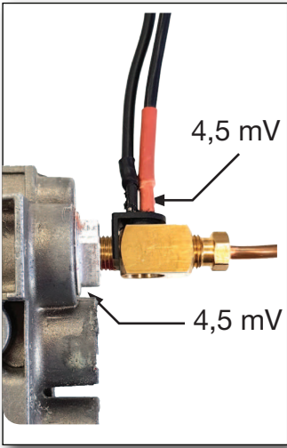
Figure A-5: interrupter
