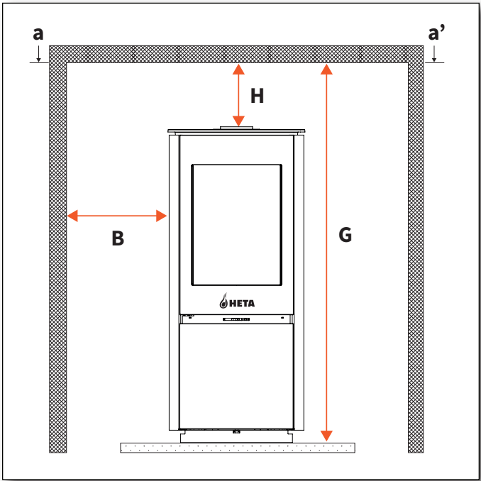
Figure 6.2 - Distances to combustible materials (front)
