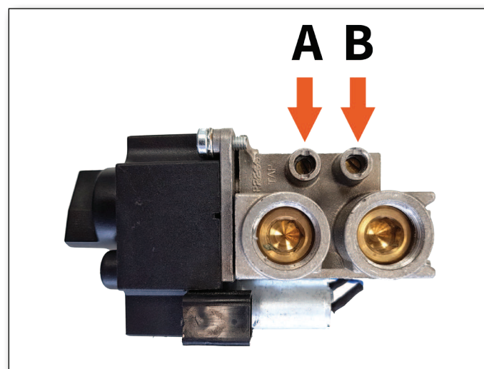
Figure 8.1 - Gas Block Measuring Points
