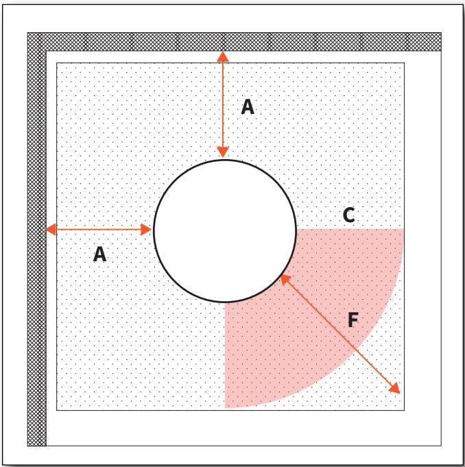
Figure 6.1 - Distances to combustible materials (top)
